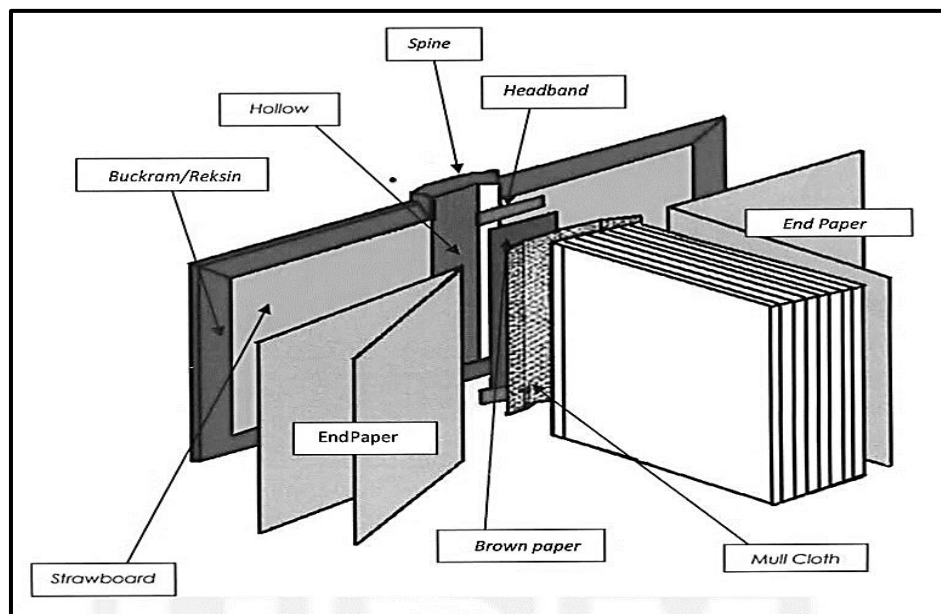
Rajah 7: Kaedah Penjilidan Kulit Keras
